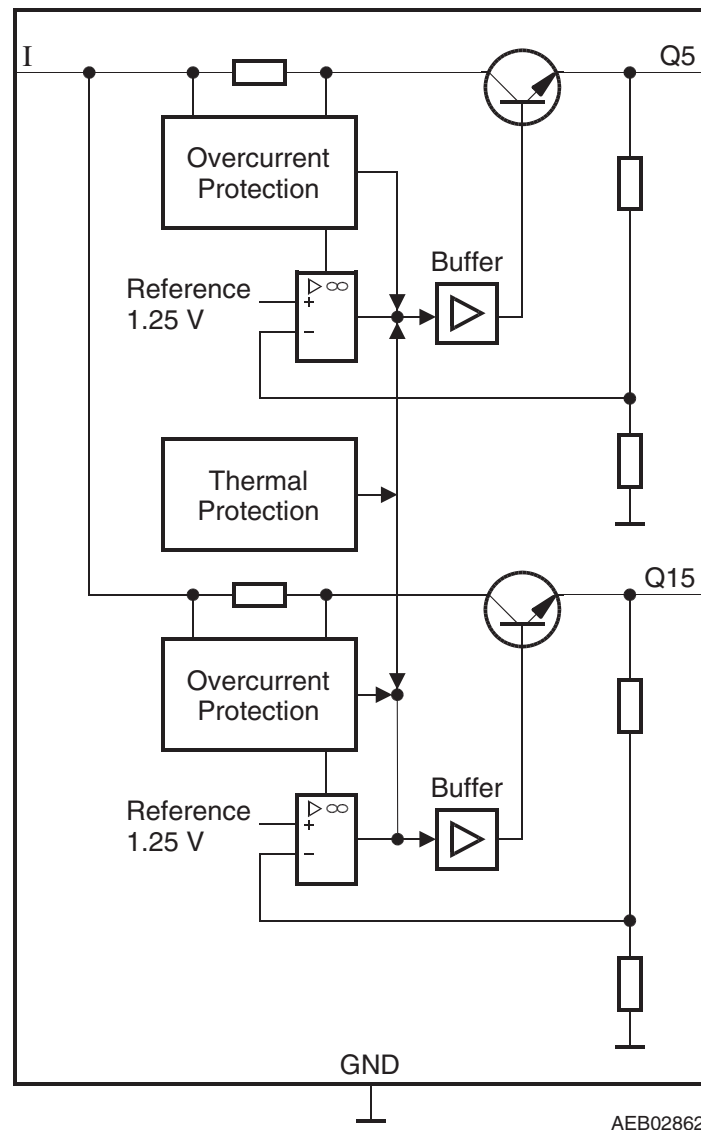
Figure 2 Block Diagram
