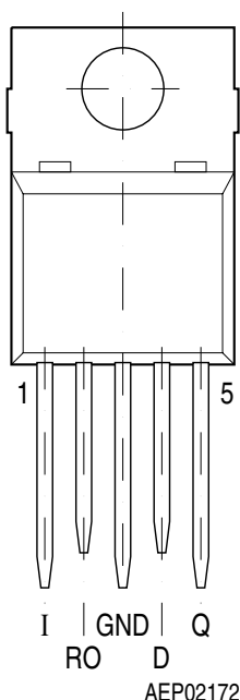
Figure 1 Pin Configuration (top view)
