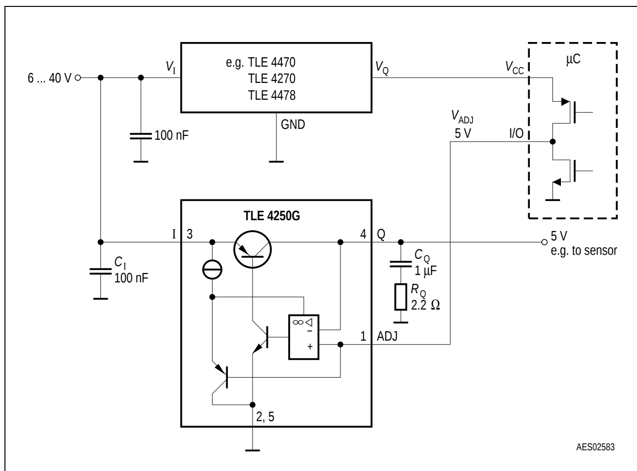
Figure 3 Application Circuit
