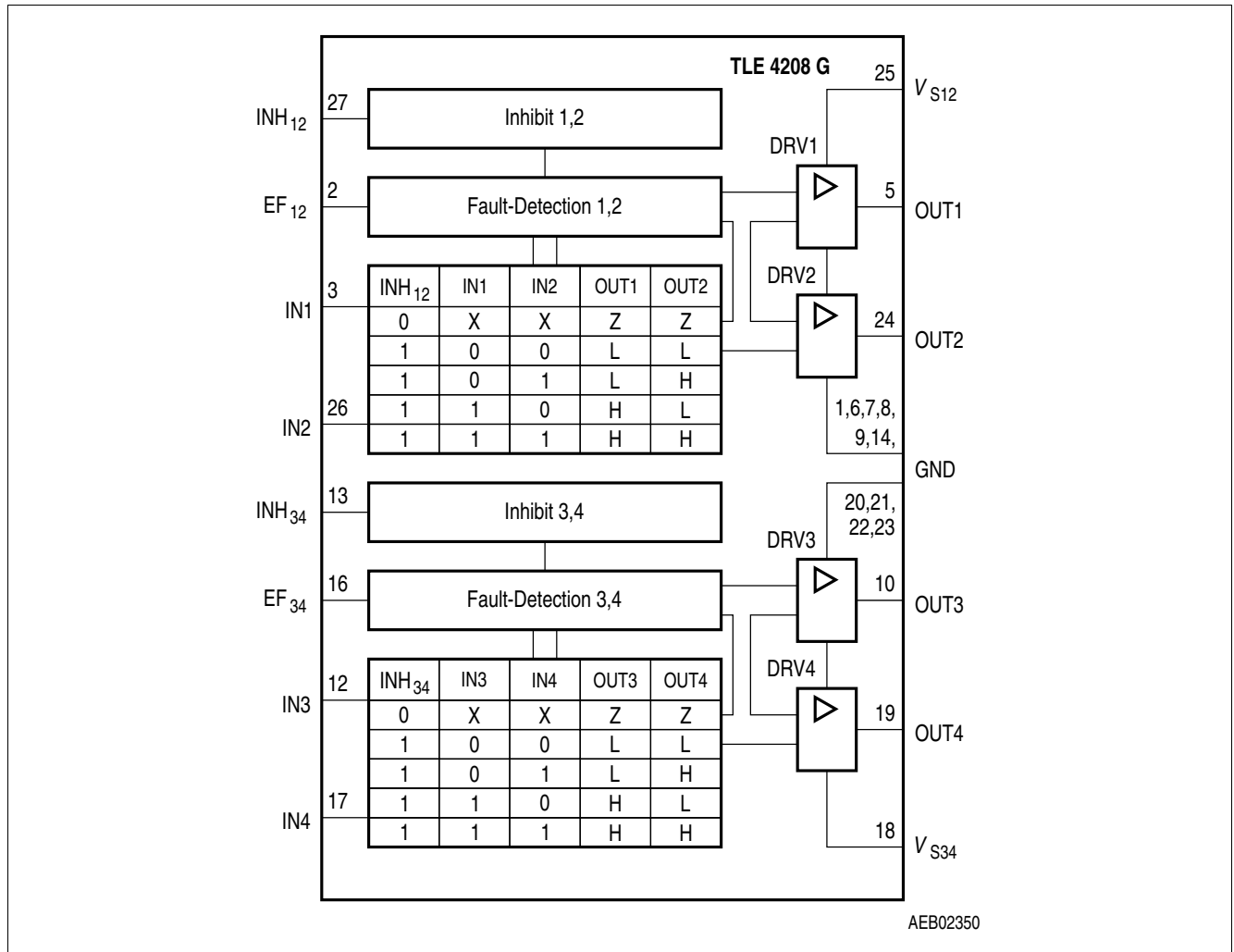
Figure 1 Block Diagram
