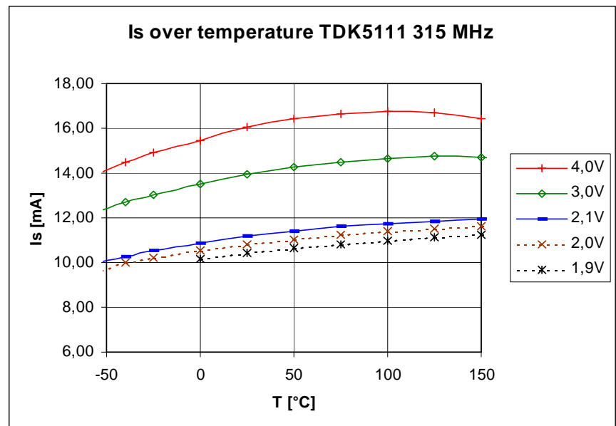
Figure 4-5 Is over temperature of the 50 \Omega -testboard with TDK5111 at 315 MHz
