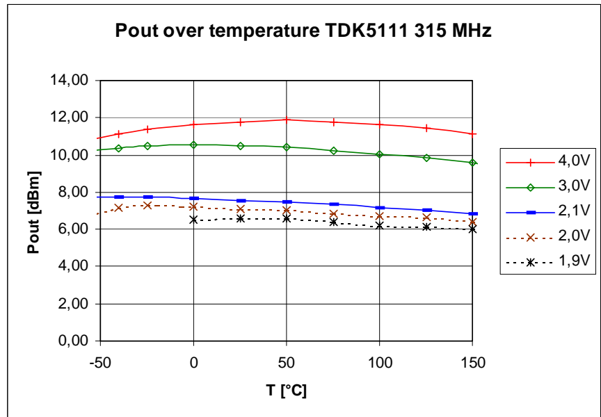
Figure 4-4 Pout over Temperature of the 50 \Omega -testboard with TDK5111 at 315 MHz
