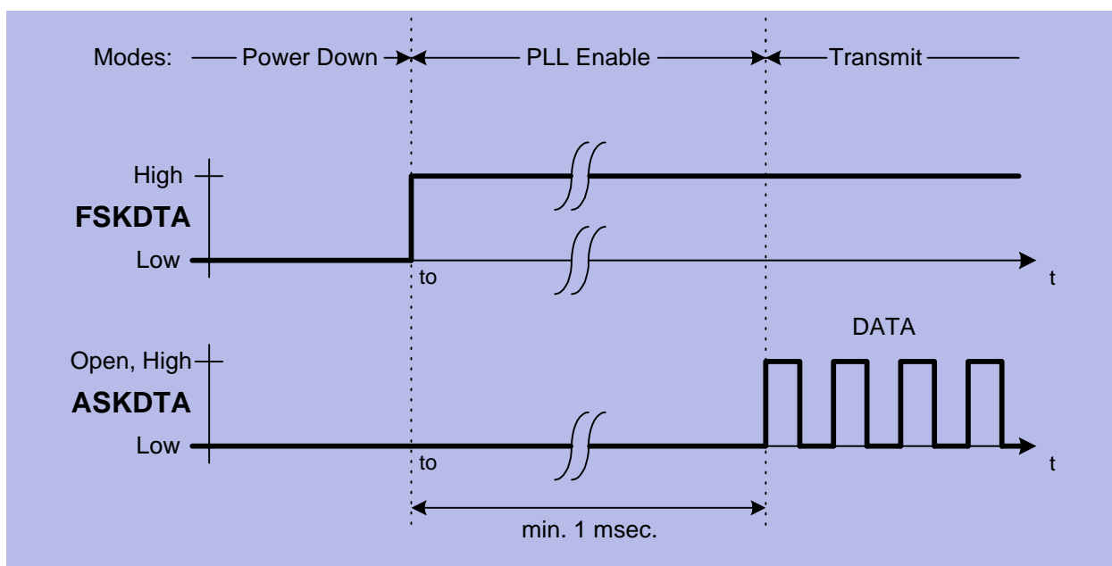
Figure 3-6 ASK Modulation
