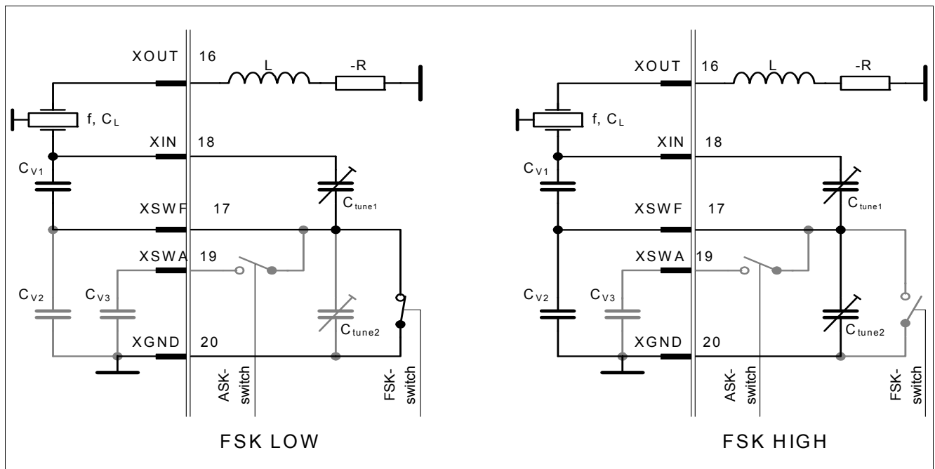
Figure 35 FSK Modulation
