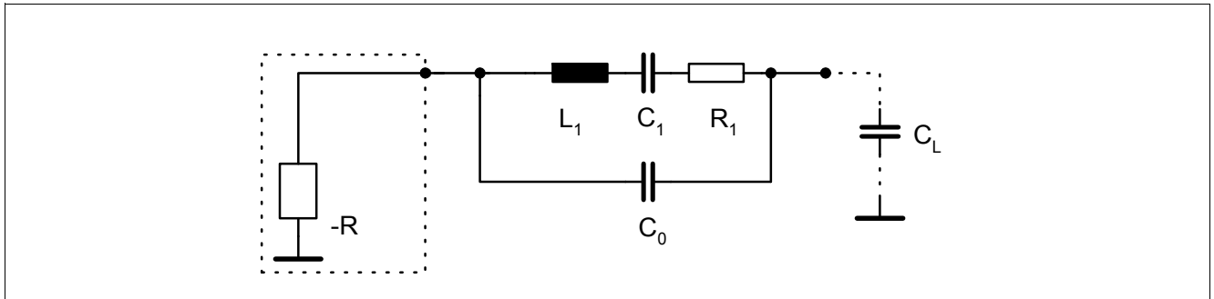
Figure 32 Crystal
