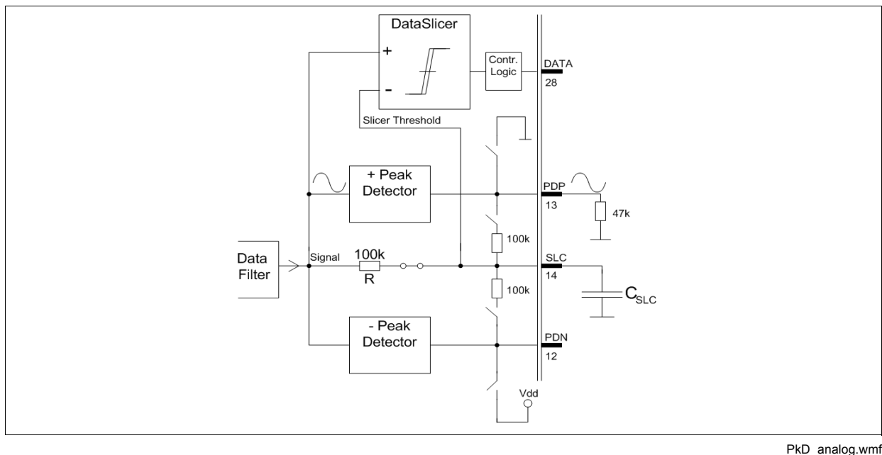
Figure 3-28 Peak Detector as analog Buffer (v=1)
