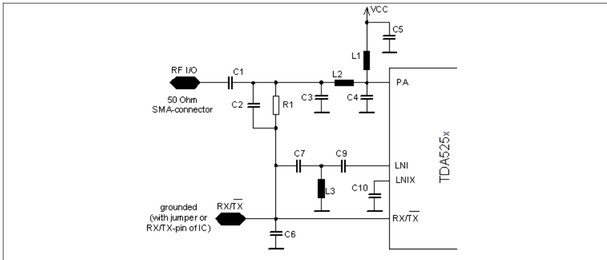
Figure 3-4 TX_Mode
