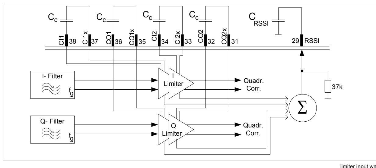
Figure 3-22 Limiter and Pinning
