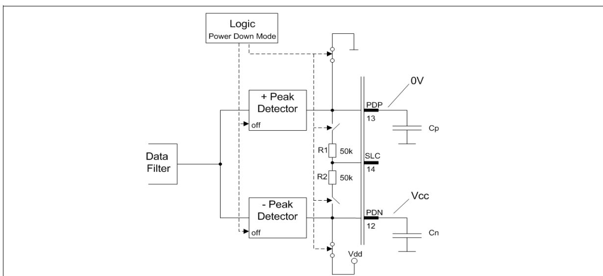
Figure 3-26 Peak detector - power down mode
