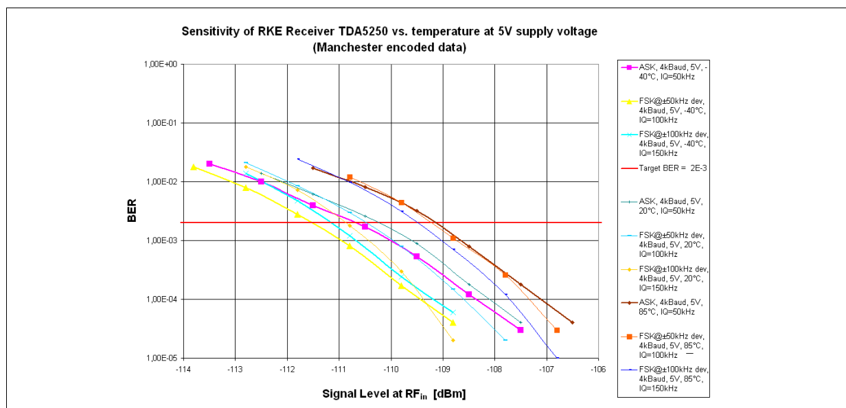
Figure 3-37 Temperature Behaviour
