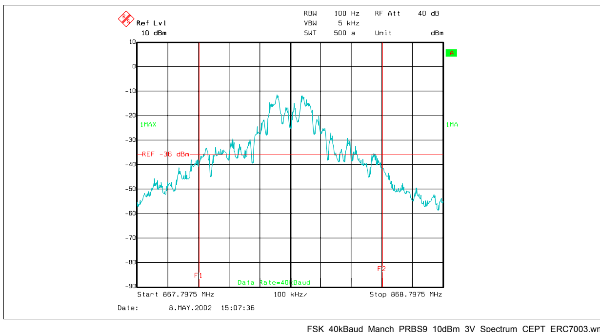
Figure 3-13 FSK Transmit Spectrum 40kBaud, Manch, PRBS9, 9dBm, 3V
