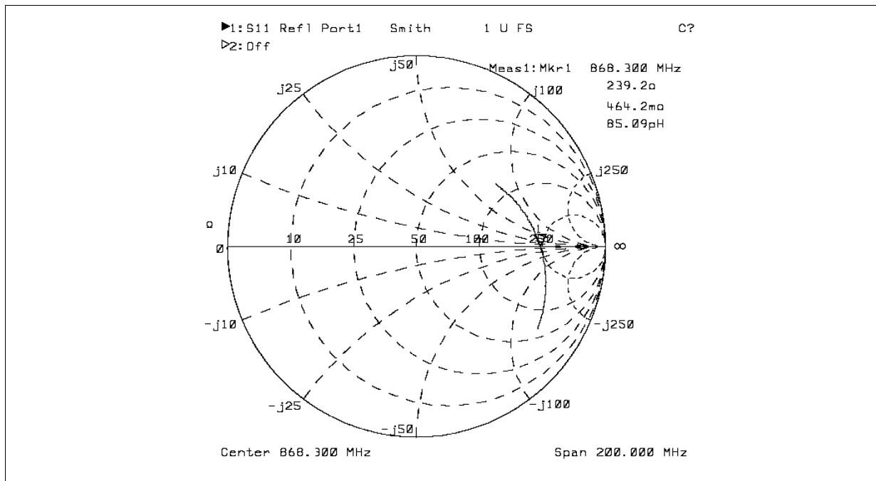
Figure 3-9 Sparam_measured_200M
