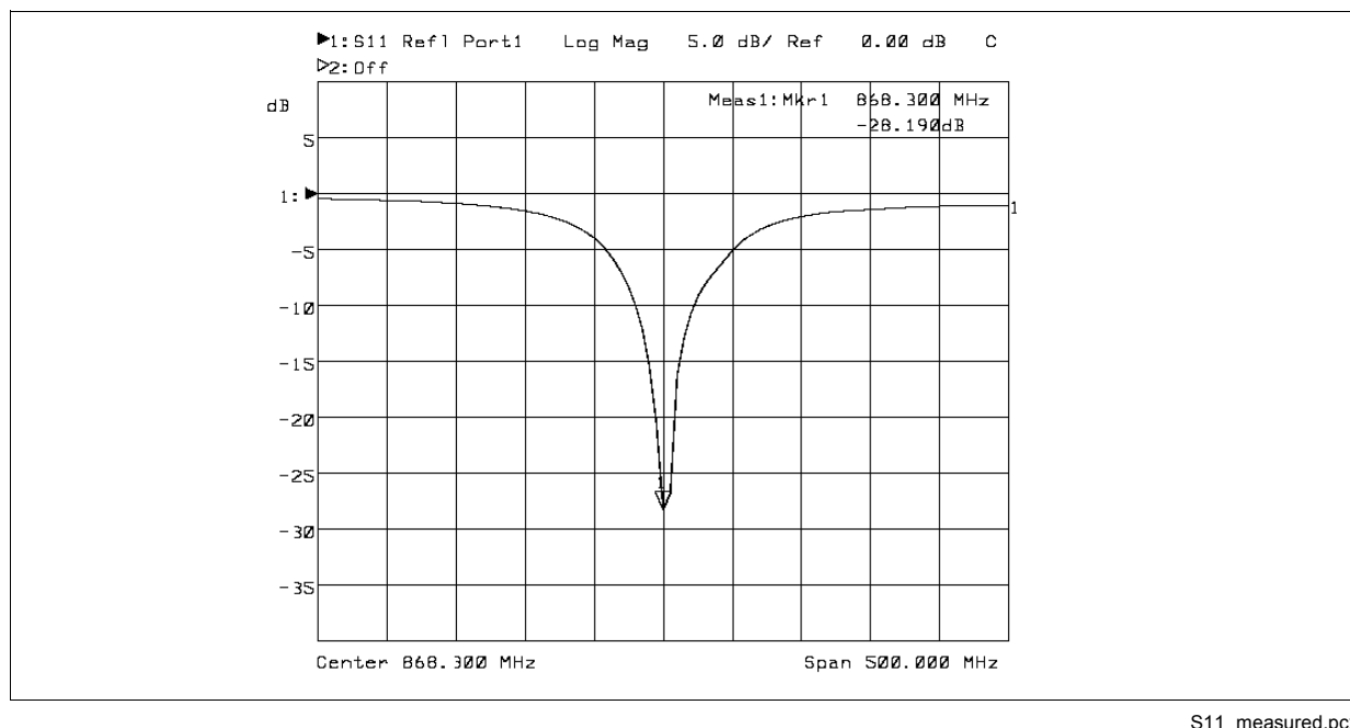
Figure 3-3 S11 measured
