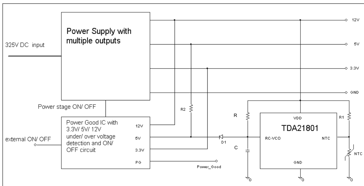
Fig. 4 OTP Application circuit
