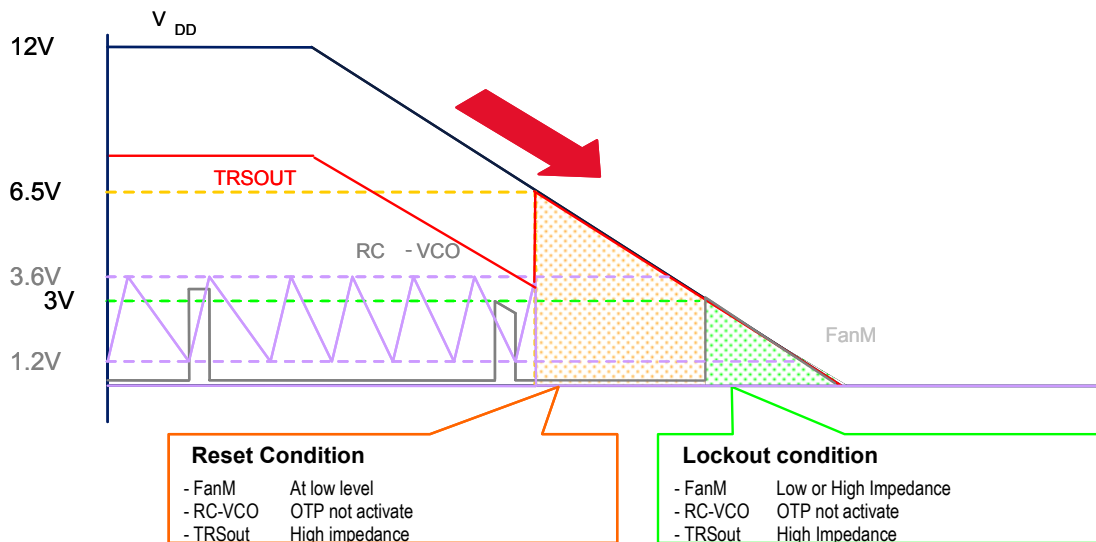
Fig.13 Power Down main waveforms transitory
