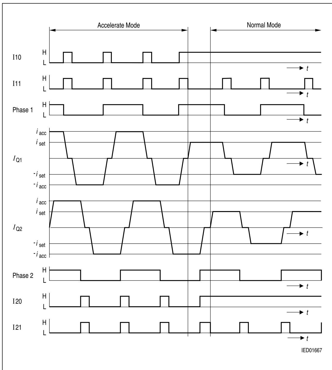
Figure 8 Half-Step Operation
