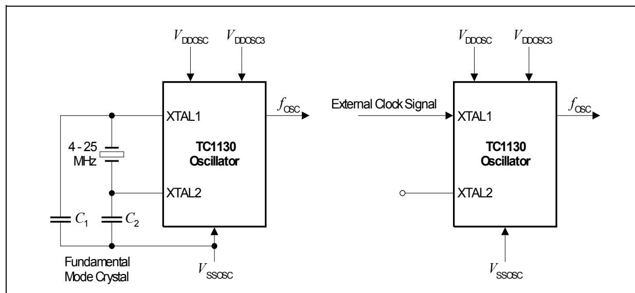
Figure 3-17 Oscillator Circuitries
