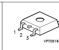
P-TO263-3-2
