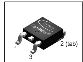
PG-TO252-3-11
