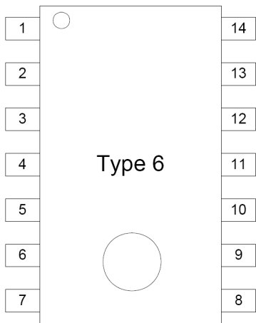
Figure 3: Pin Configuration. Top view, not to scale
