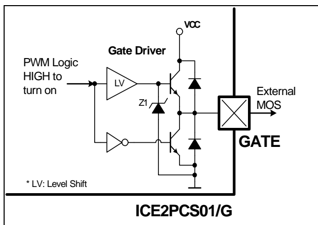
Figure 16 Gate Driver
