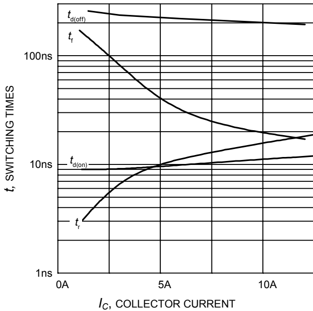
Figure 9. Typical switching times as a function of collector current (inductive load, T_J=150^\circ\text{C} , V_{CE}=400\text{V} , V_{GE}=0/15\text{V} , R_G=50\Omega , Dynamic test circuit in Figure E)
