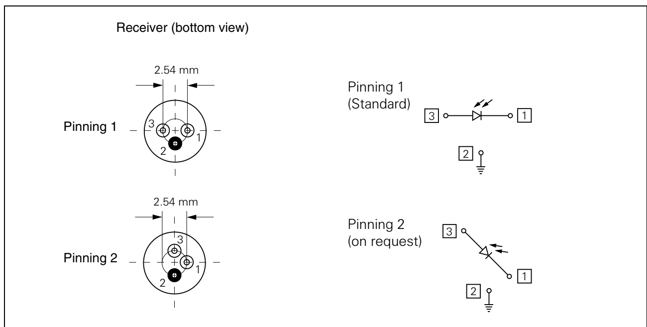
Figure 2 Receiver
