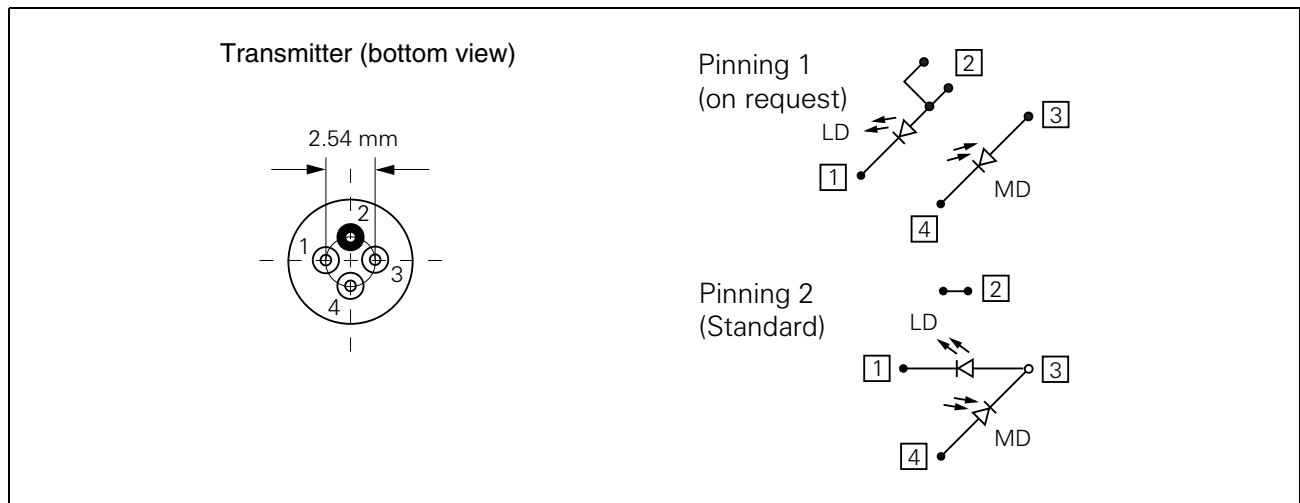
Figure 1 Transmitter
