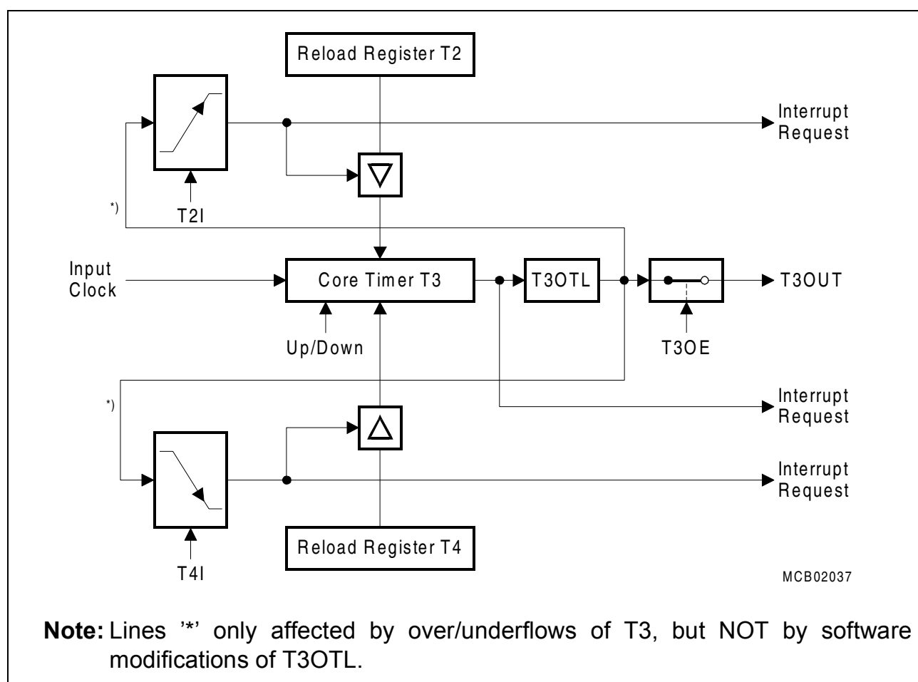
Figure 69 GPT1 Timer Reload Configuration for PWM Generation
