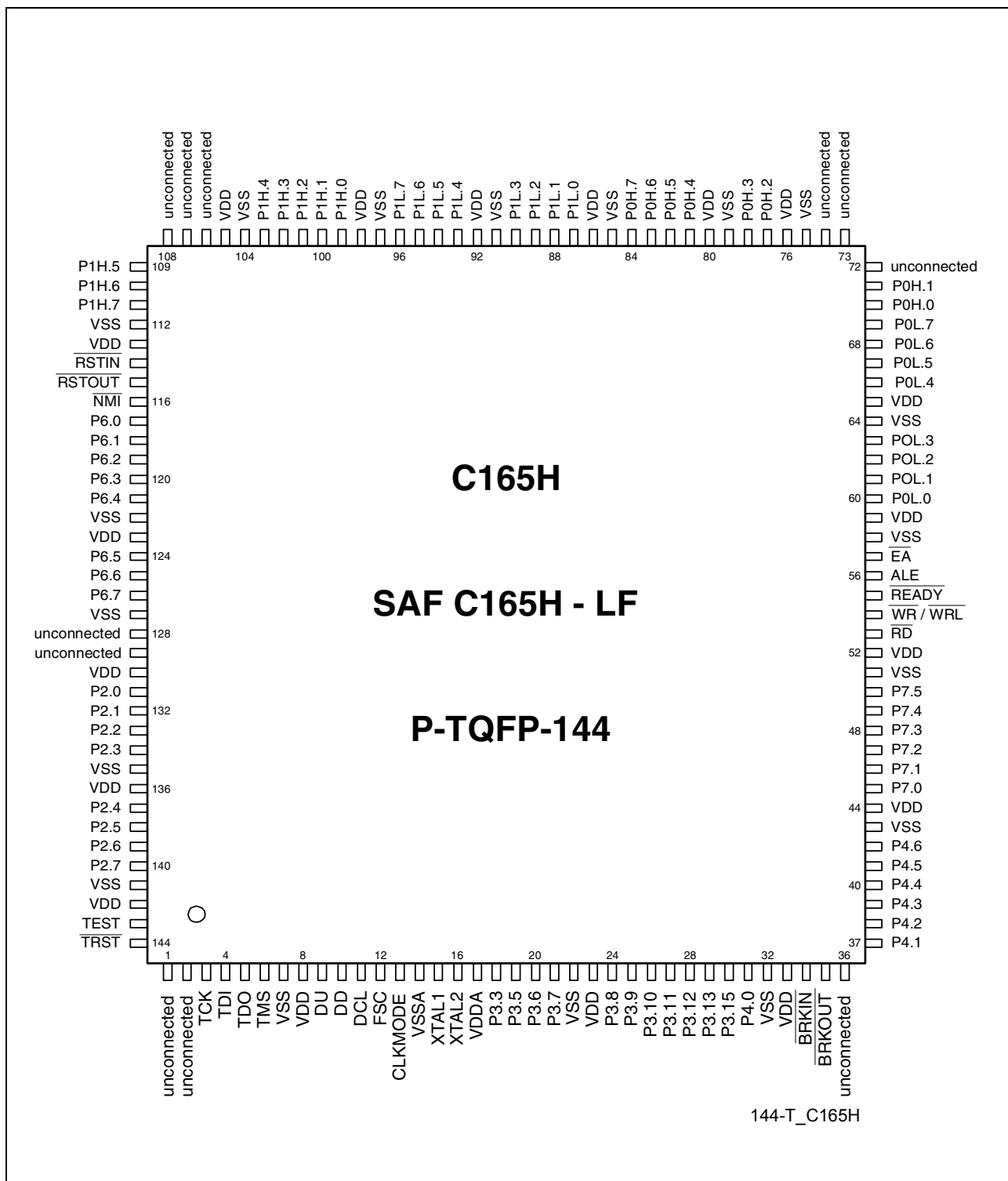
Figure 2 Pinning Diagram of the C165H
