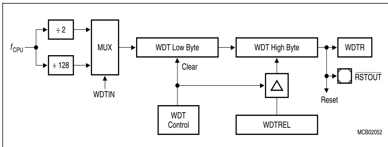
Figure 126 Watchdog Timer Block Diagram
