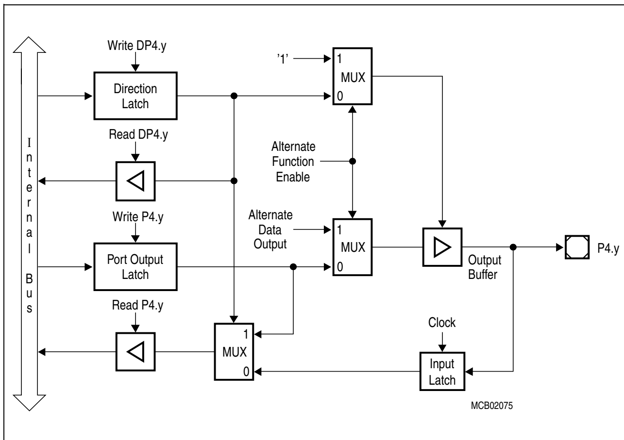
Figure 38 Block Diagram of a Port 4 Pin (y = 6...0)
