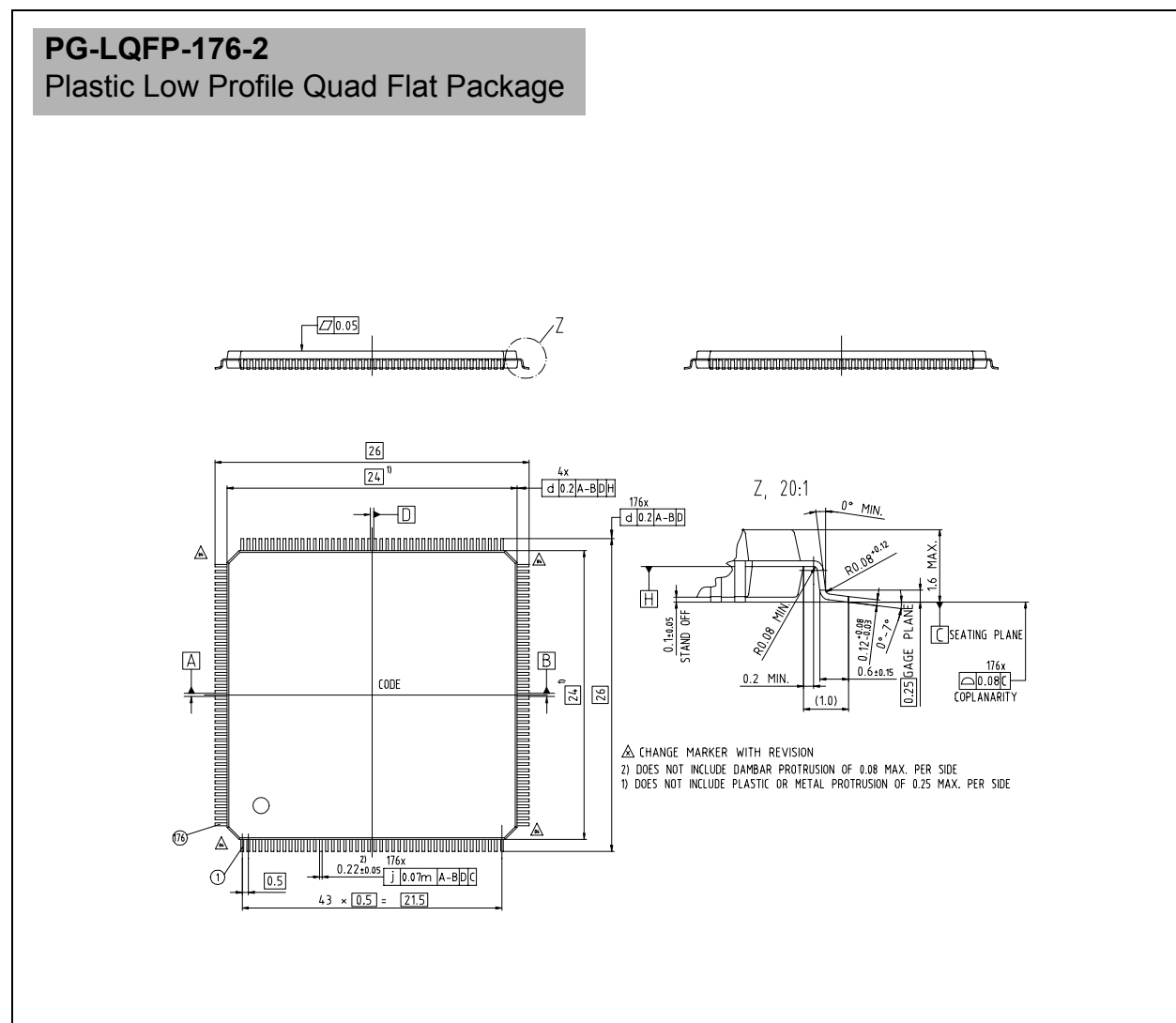
Figure 5-1 Package Outlines PG-LQFP-176-2
