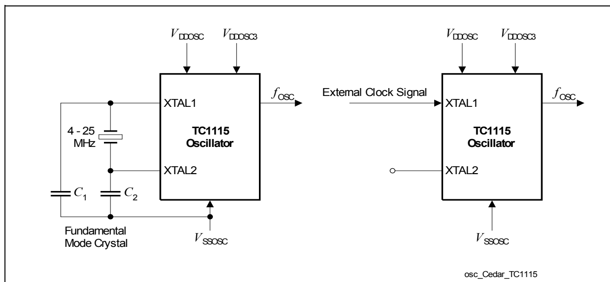
Figure 3-15 Oscillator Circuitries
