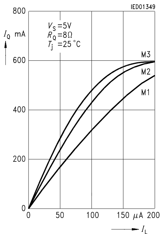
Peak Current I_Q versus Loudness-Current I_L
