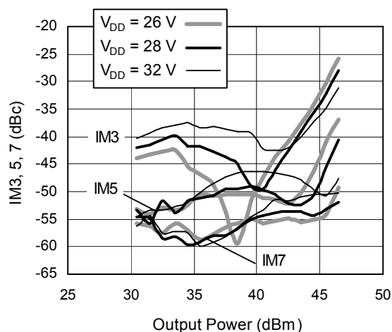
Two-tone Performance, various voltages
