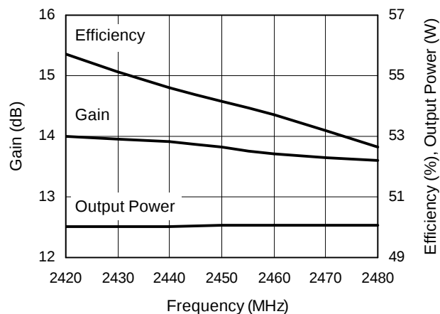
Typical P_{OUT} , Gain & Efficiency (at P-1dB) vs. Frequency
