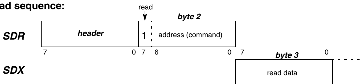
Figure 8 Serial Command Structure
