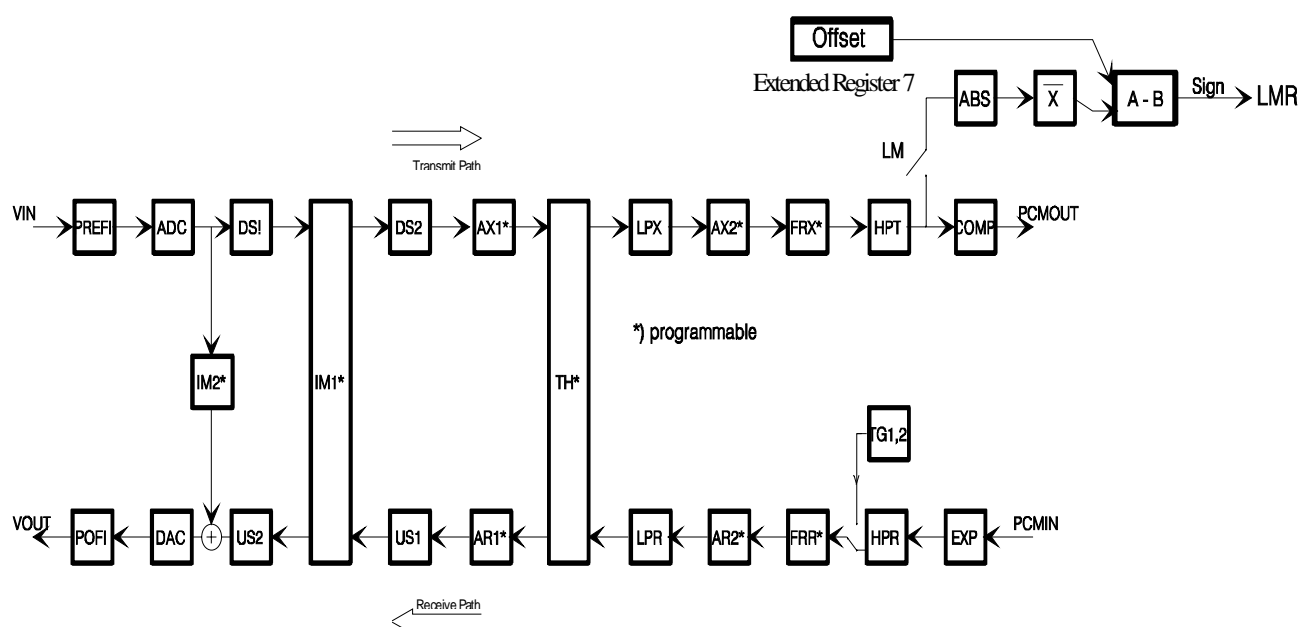
Figure 30 Block diagram of one SICOI2/4-TE channel
