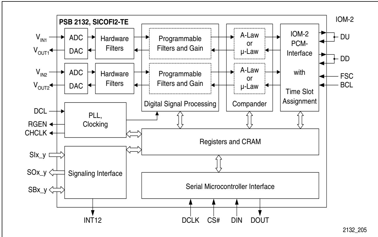
Figure 4 SICOPI2-TE Block Diagram
