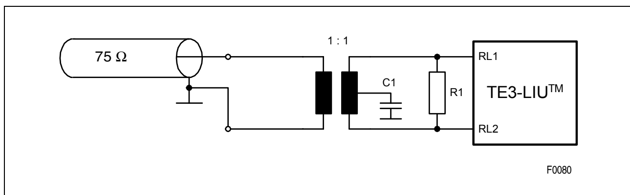
Figure 7 Receiver Configuration
