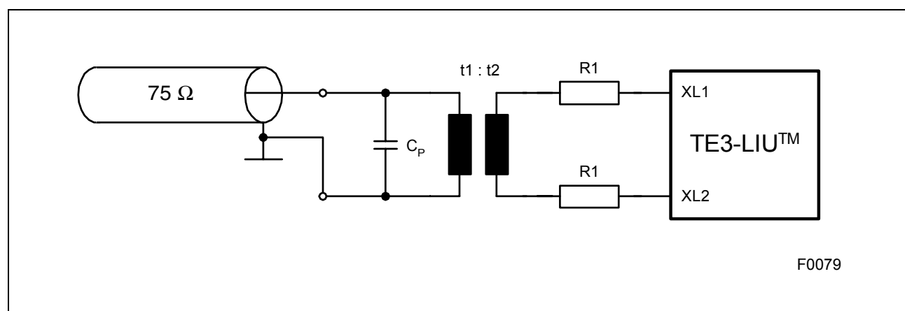
Figure 13 Transmitter Configuration
