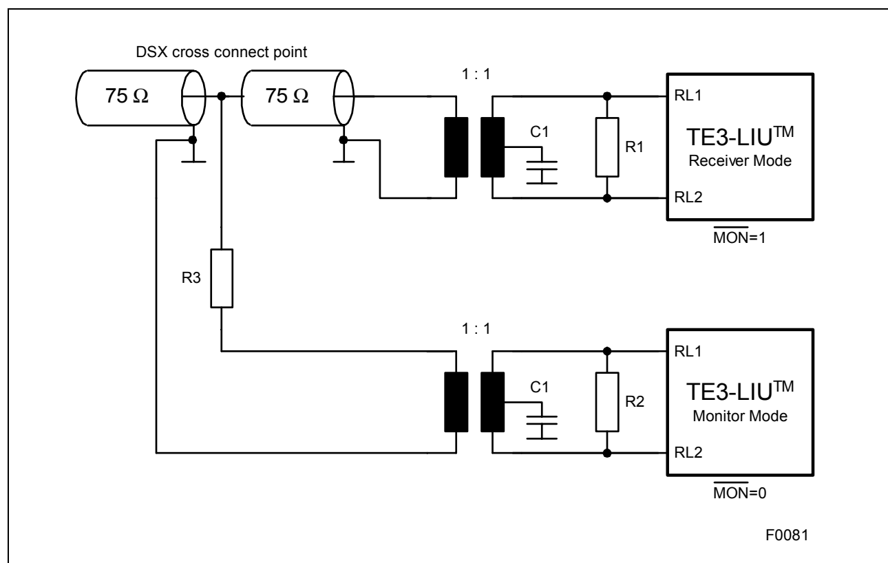
Figure 8 DS3 Line Monitoring
