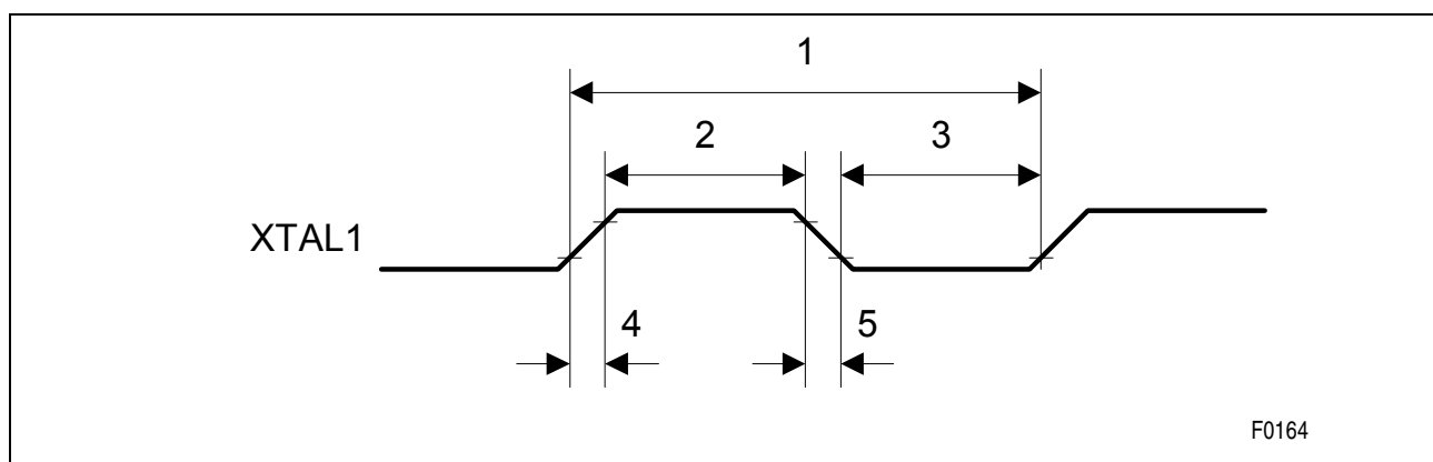
Figure 20 XTAL Clock Timing
