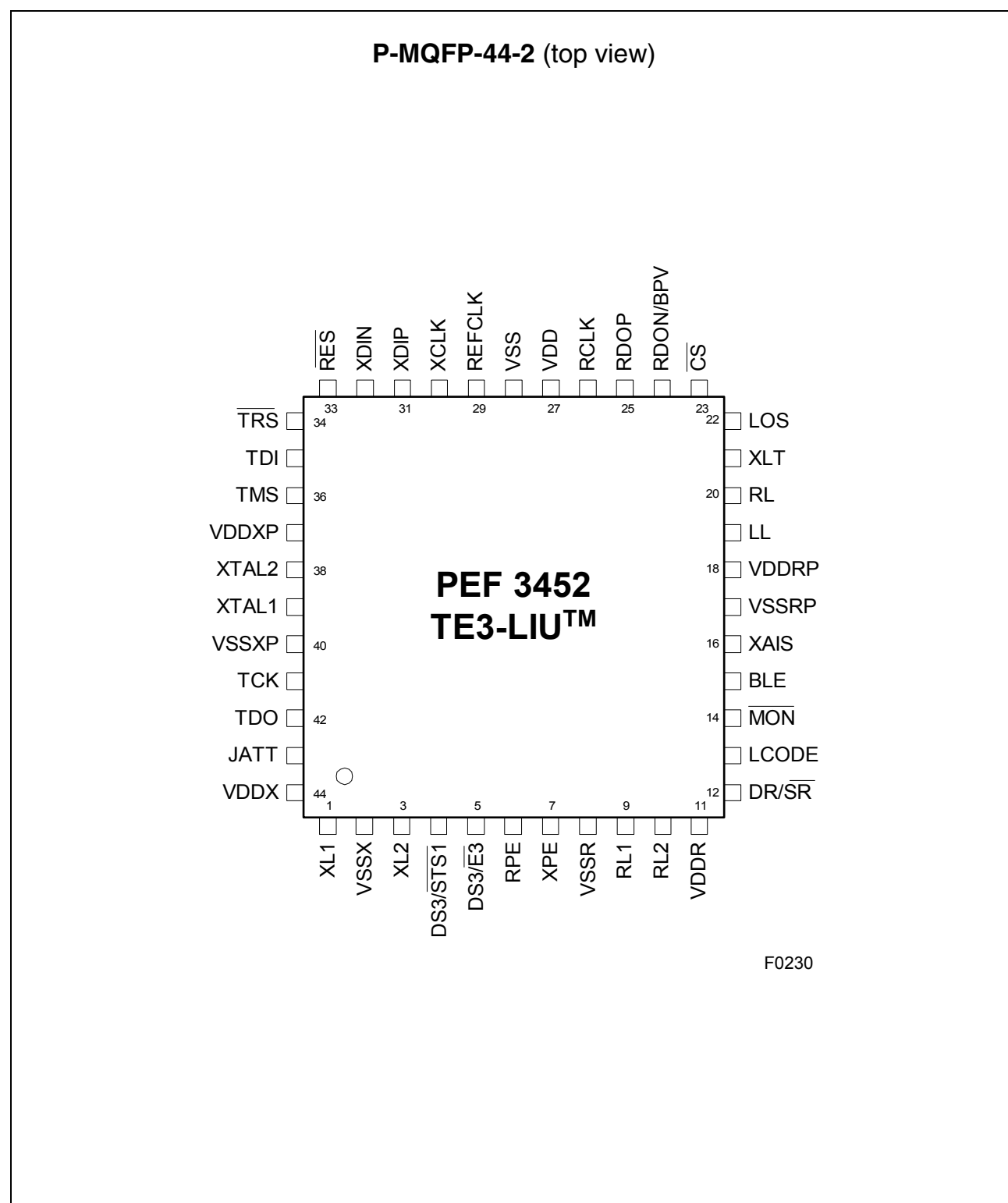
Figure 5 Pin Configuration
