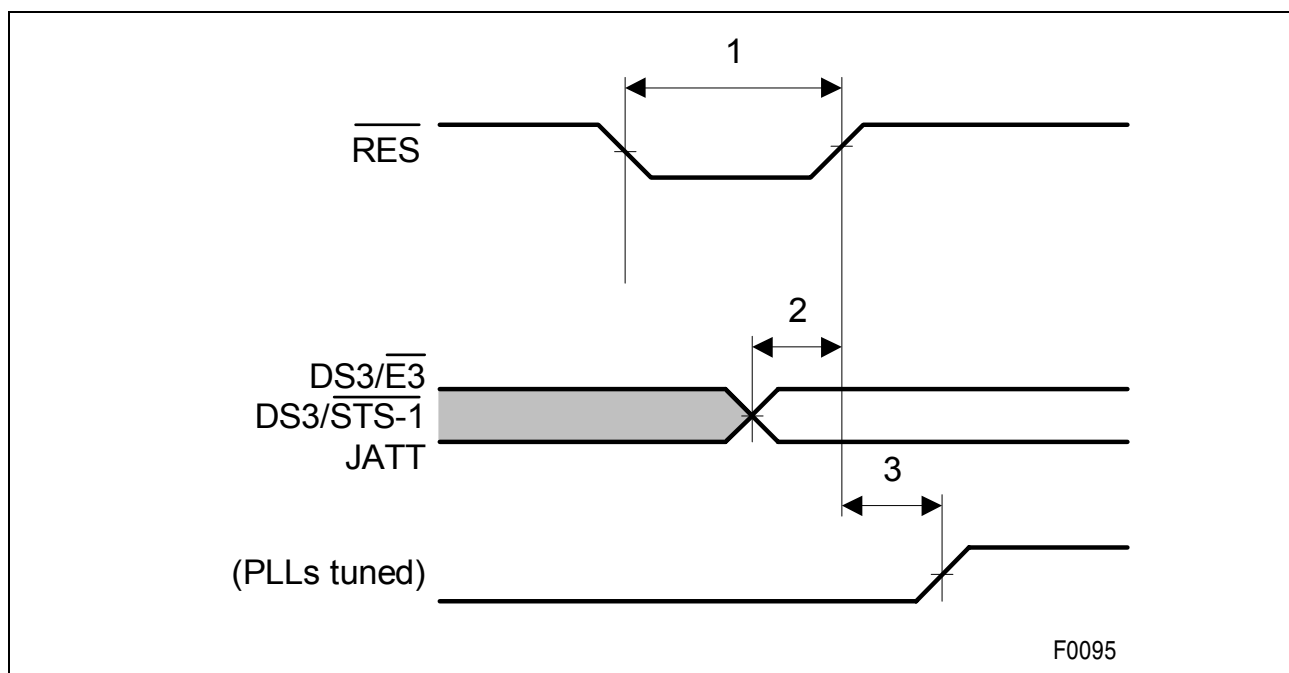
Figure 18 Reset Timing
