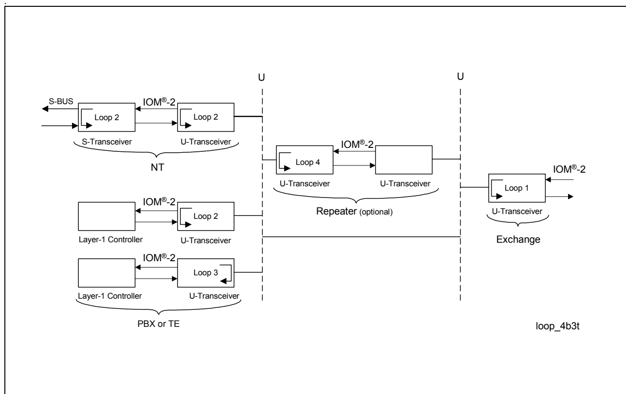
Figure 26 Test Loopbacks
