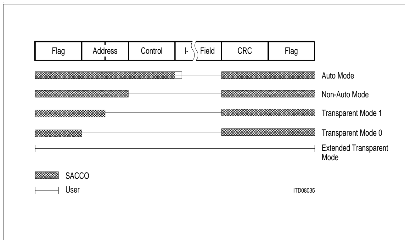
Figure 35 Support of the HDLC Protocol by the SACCO
