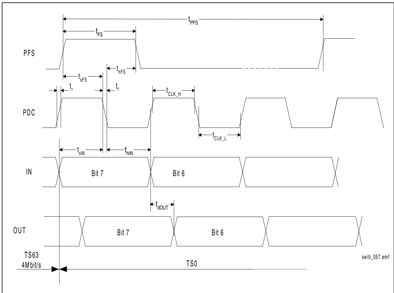
Figure 31 PCM Timing
