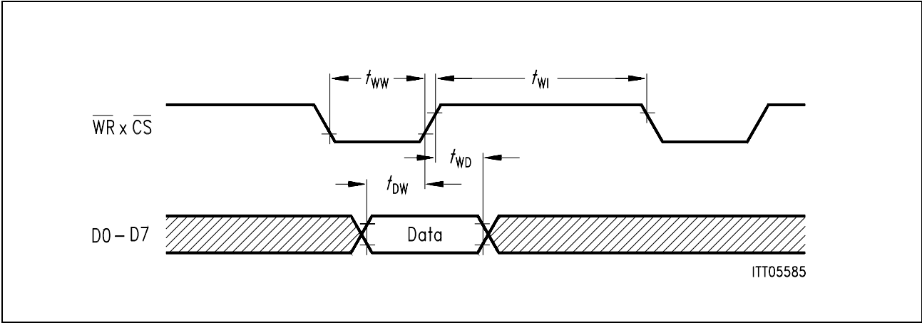
Figure 16 \mu\text{P} Write Cycle
