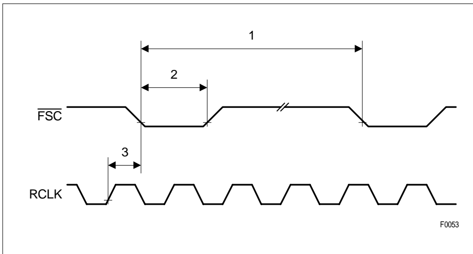
Figure 32 FSC Timing
