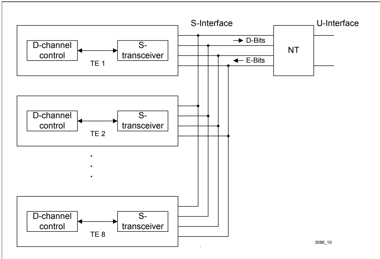
Figure 68 D-Channel Access Control on the S-Interface
