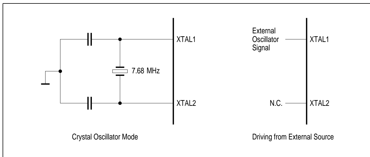
Figure 68 Oscillator Circuits
