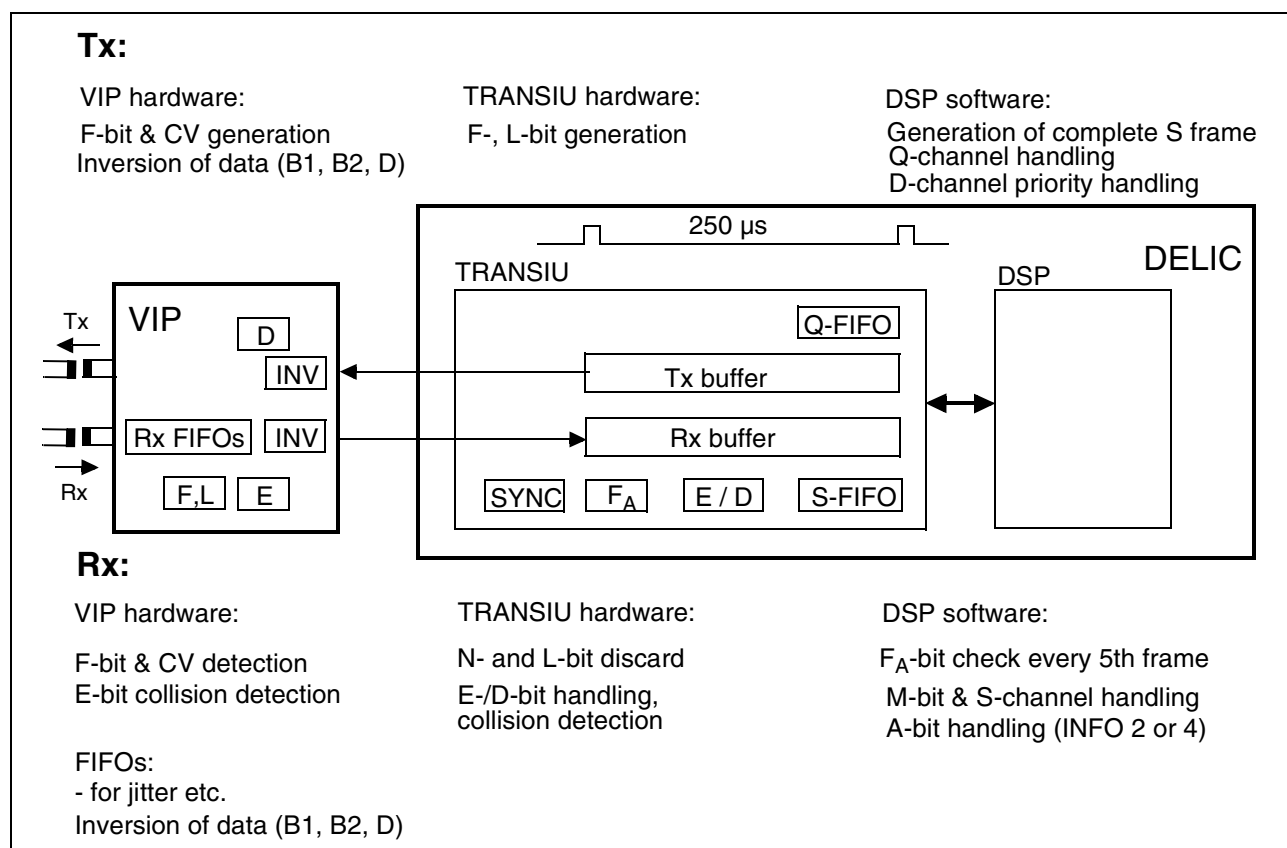
Figure 30 Handling of So Frame in LT-T Mode (One Channel)
