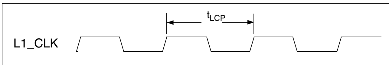
Figure 89 L1_CLK Timing
