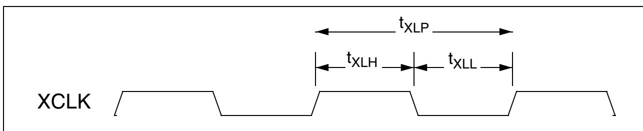
Figure 90 XCLK Timing
