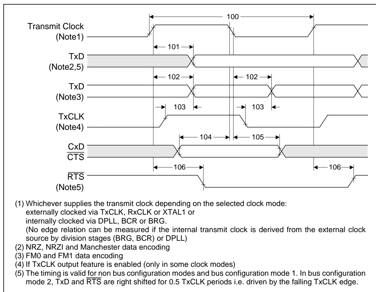
Figure 81 Transmit Cycle Timing
