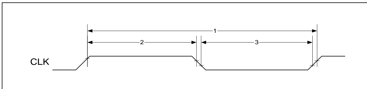
Figure 69 Microprocessor Interface Clock Timing
