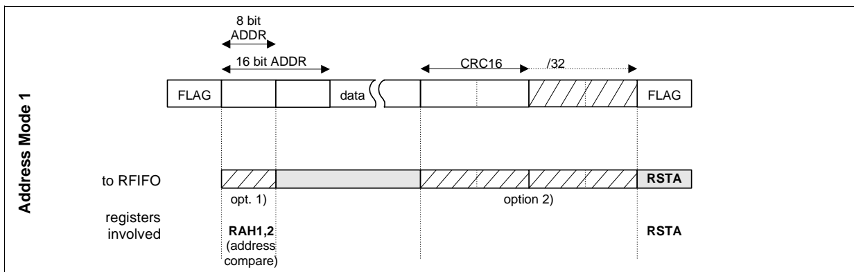
Figure 45 HDLC Receive Data Processing in Address Mode 1
