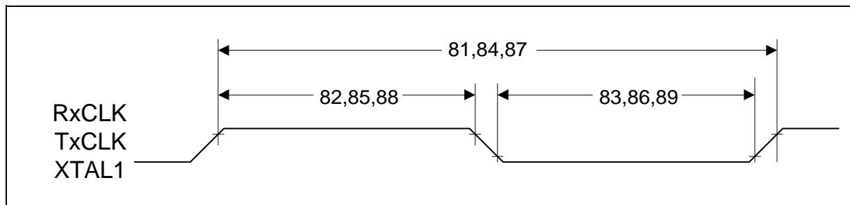
Figure 79 Clock Input Timing
