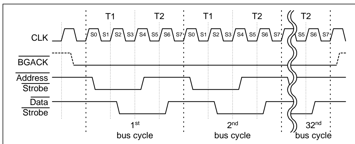
Figure 37 Un-interrupted Series of 32 DMA Bus Cycles
