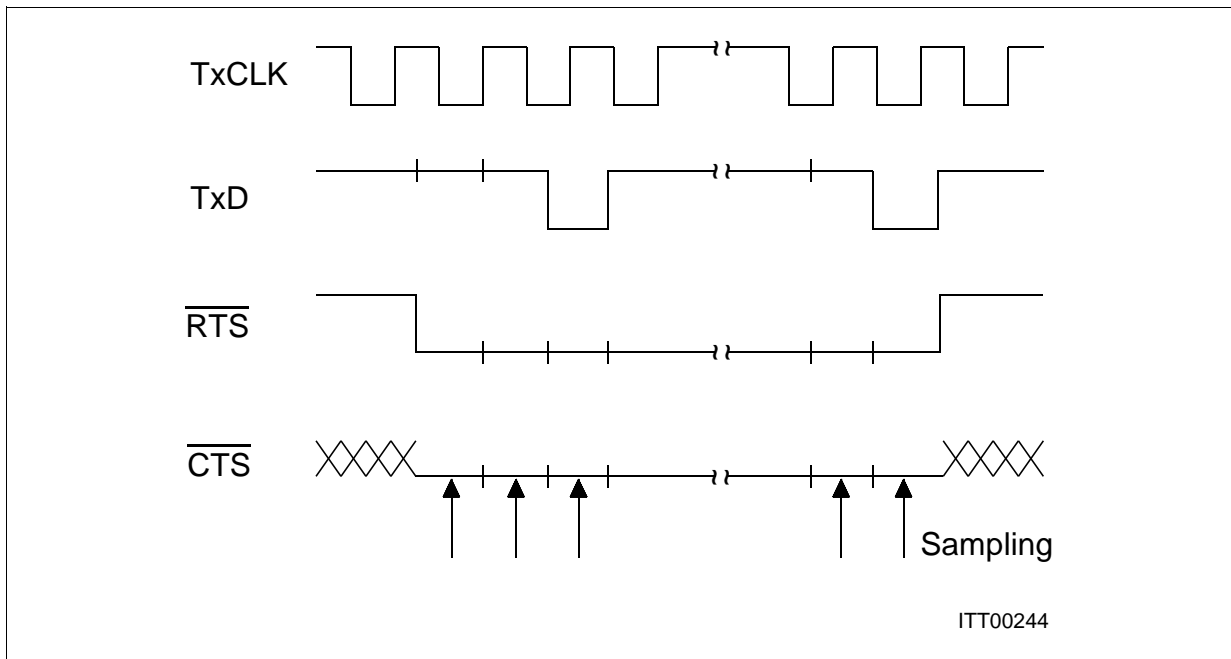
Figure 34 \overline{\text{RTS}}/\overline{\text{CTS}} Handshaking
