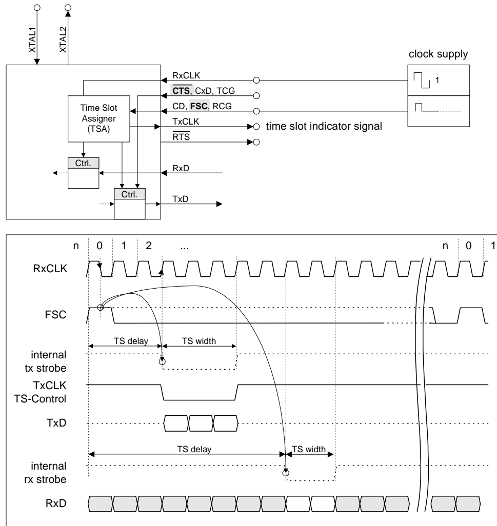
Figure 20 Clock Mode 5a Configuration
