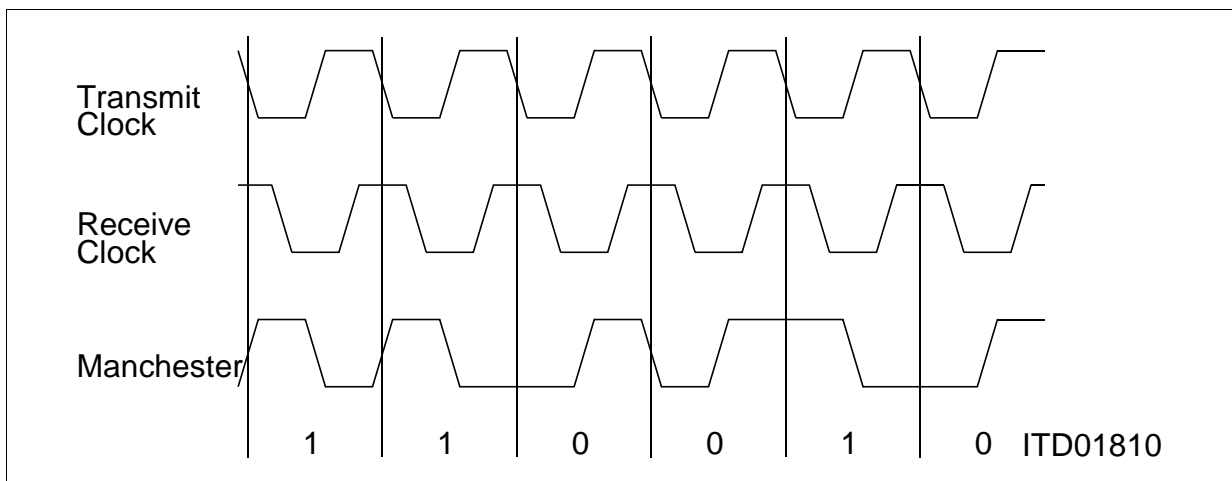
Figure 33 Manchester Data Encoding
