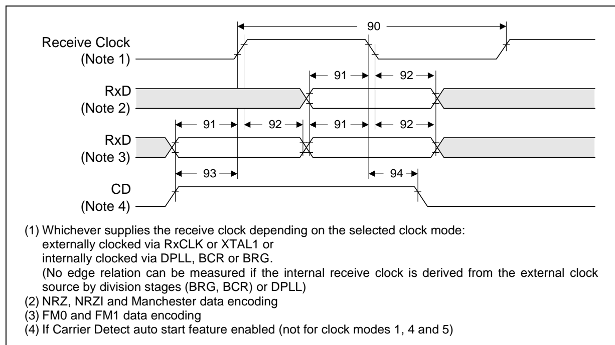
Figure 80 Receive Cycle Timing
