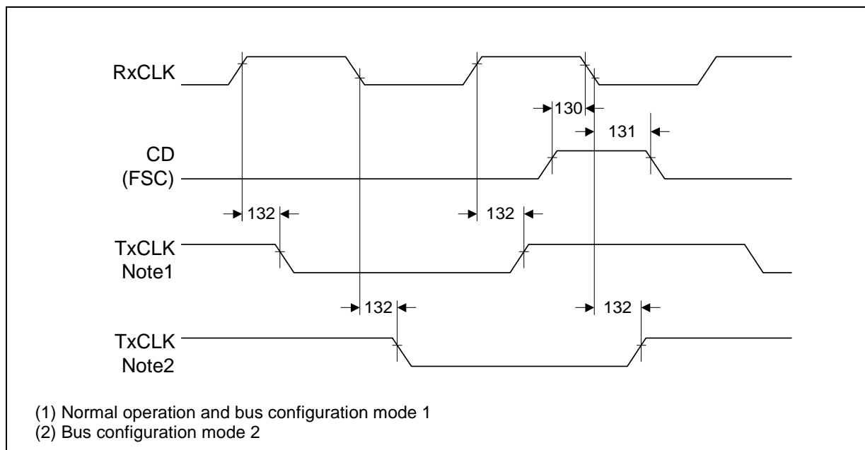
Figure 85 Clock Mode 5 Frame Synchronisation Timing
