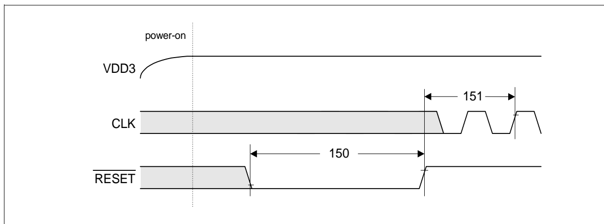
Figure 86 Reset Timing
