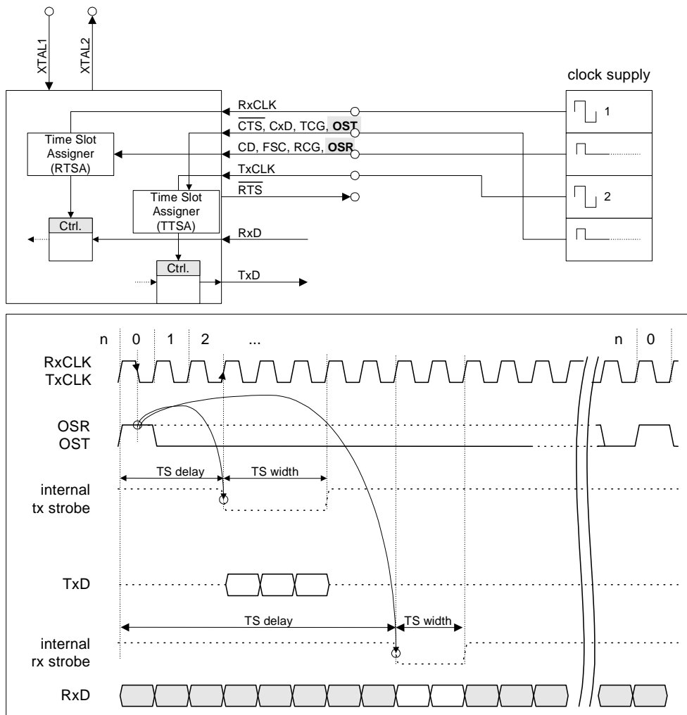
Figure 24 Clock Mode 5b Configuration
