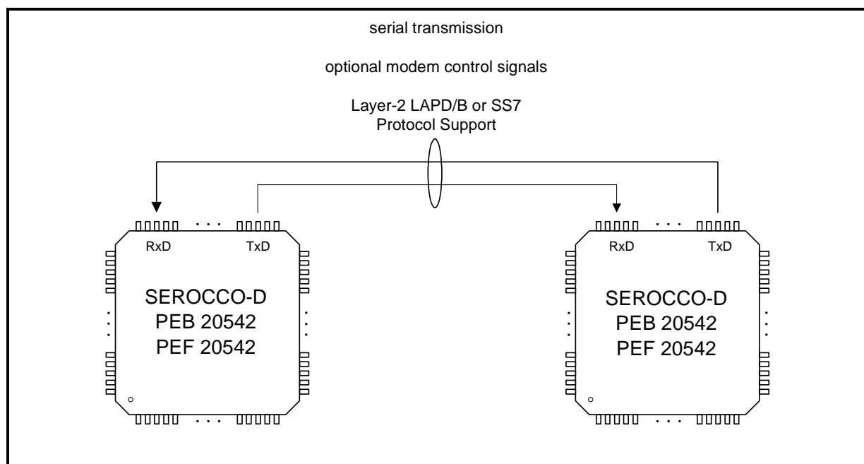
Figure 3 Point-to-Point Configuration
