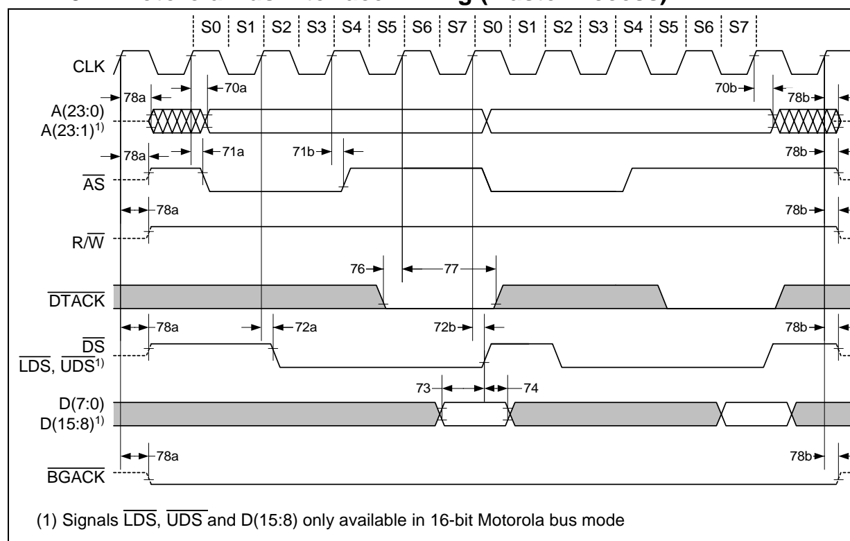
Figure 76 Motorola Read Cycle Timing (Master Access)
