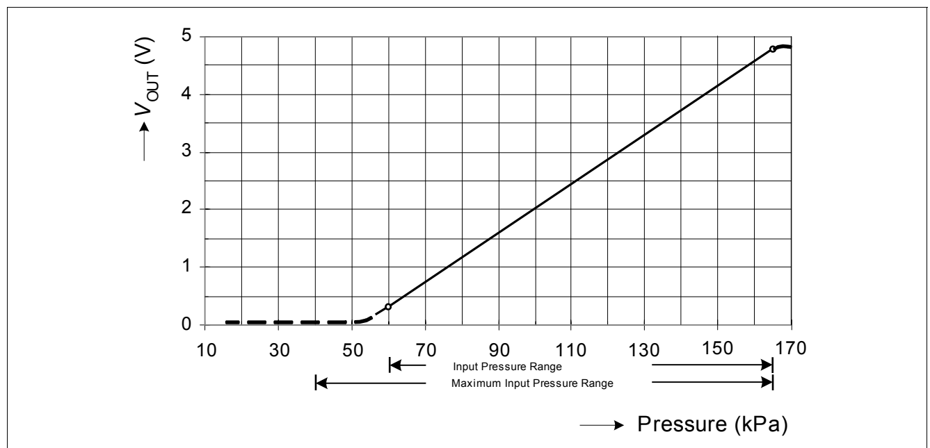
Figure 3 Transfer Function
