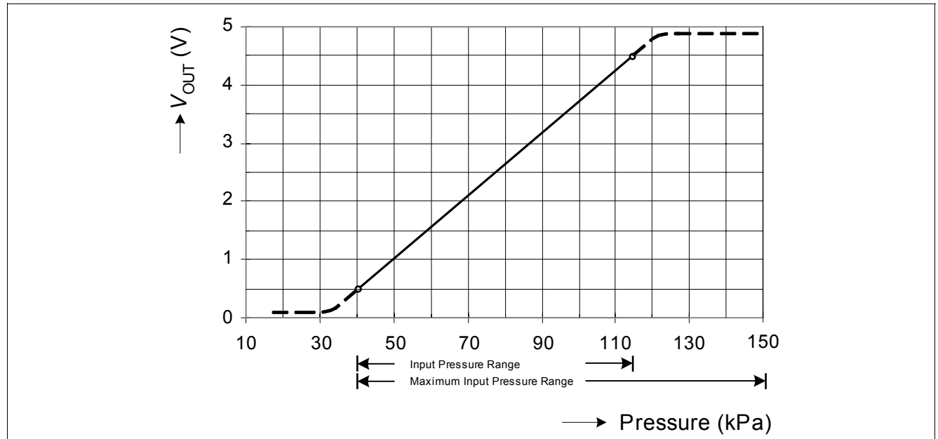
Figure 3 Transfer Function
