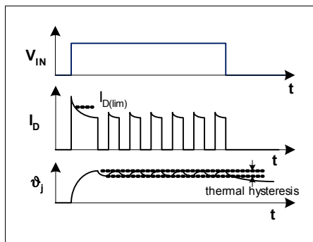
Figure 11 Short circuit
