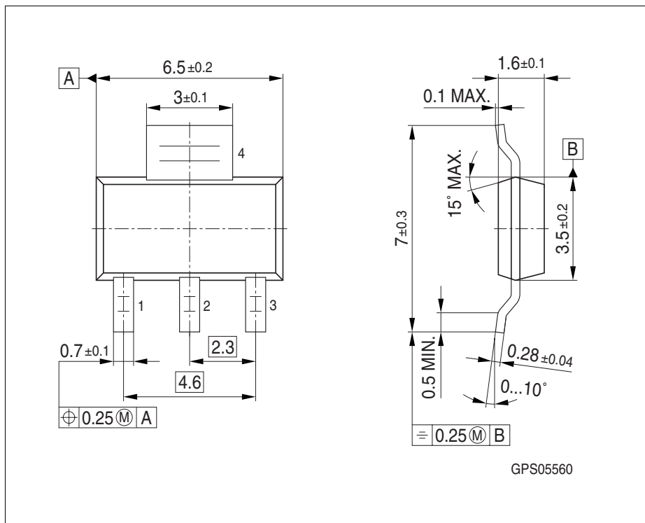
Figure 12 PG-SOT223-4
