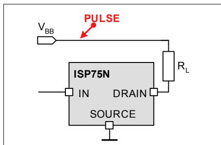
Figure 3 Test circuit for ISO pulse
