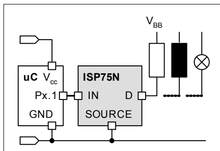
Figure 8 Application Circuit
