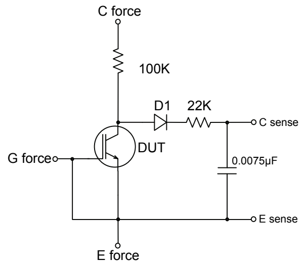
Fig.C.T.6 - BVCE Filter Circuit
