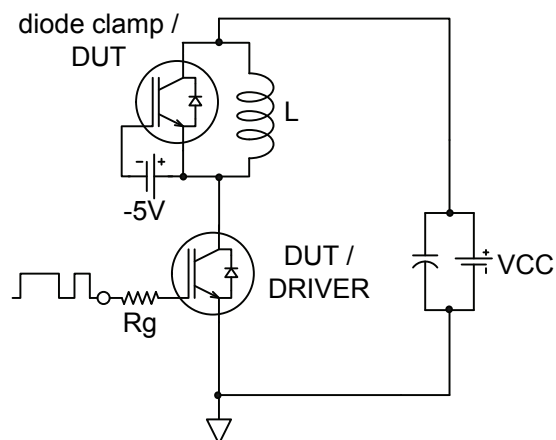
Fig.C.T.2 - RBSOA Circuit
