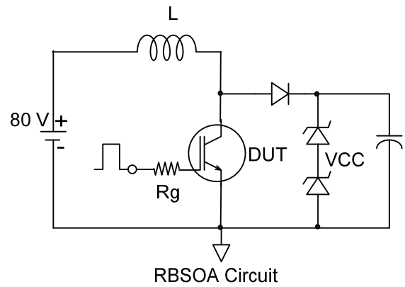
Fig.C.T.2 - RBSOA Circuit
