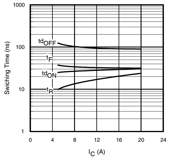
Fig. 14 - Typ. Switching Time vs. I_C T_J = 175^\circ\text{C} ; L = 1\text{mH} ; V_{CE} = 400\text{V} R_G = 22\Omega ; V_{GE} = 15\text{V}
