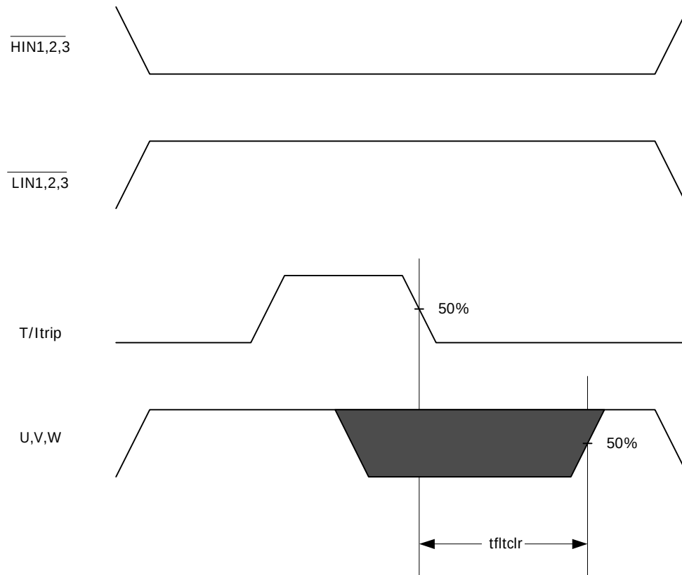
Figure 2. I_{\text{Trip}} Timing Waveform
