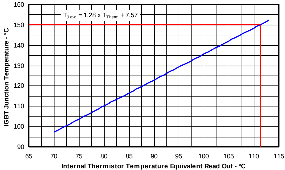
Figure 9. Estimated Maximum IGBT Junction Temperature vs. Thermistor Temperature Sinusoidal Modulation, V^+ = 400\text{V} , I_{phase} = 5\text{A}_{rms} , f_{sw} = 16\text{kHz} , f_{mod} = 50\text{Hz} , MI = 0.8 , PF = 0.6
