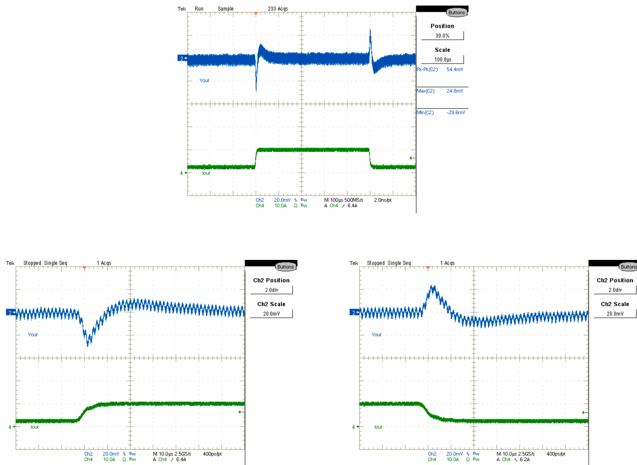
Figure 37: V_{out} Transient Response, 2.5A to 10.0A step at 2.5A/μSec CH2: V_{out} , CH4: I_{out} (10A/V)
