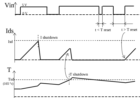
Figure 1 - Timing diagram
