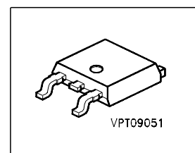
PG-TO252-3
